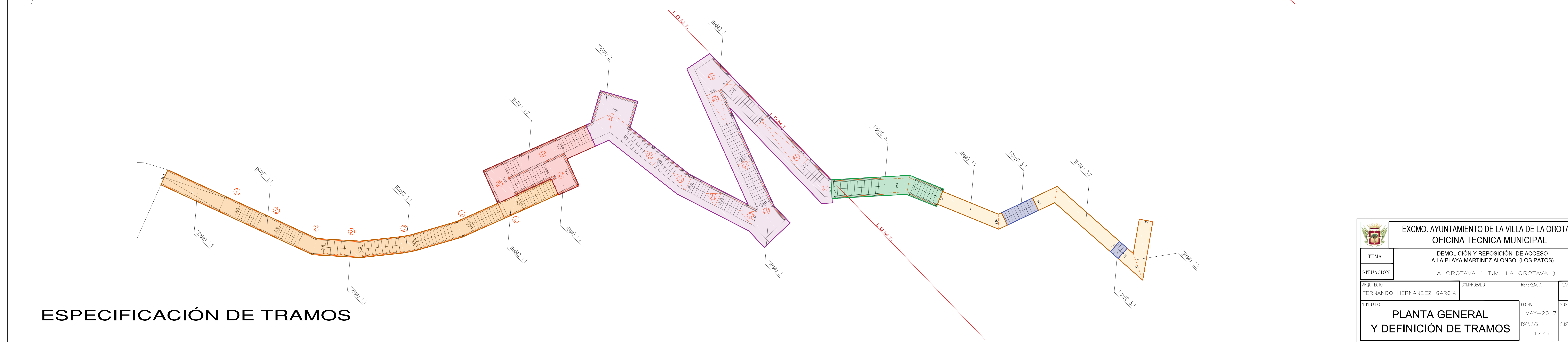
PLANTA GENERAL 1/75
